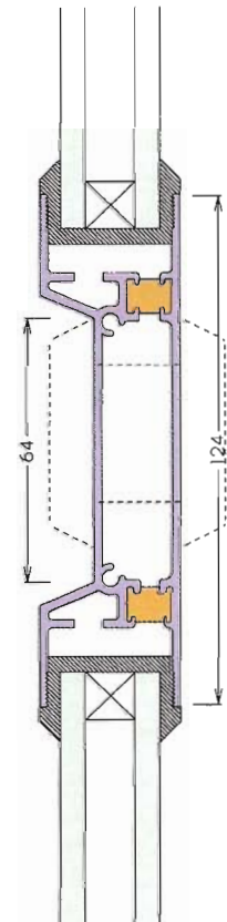
Recessed profile mid-rail - letterplate shown with broken line -
