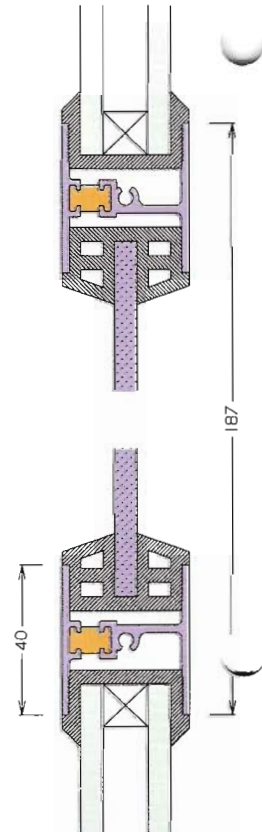
Spandrel assembly As noted, Monarch standard spandrel is 187mm high. It can be sized to suit requirements.
